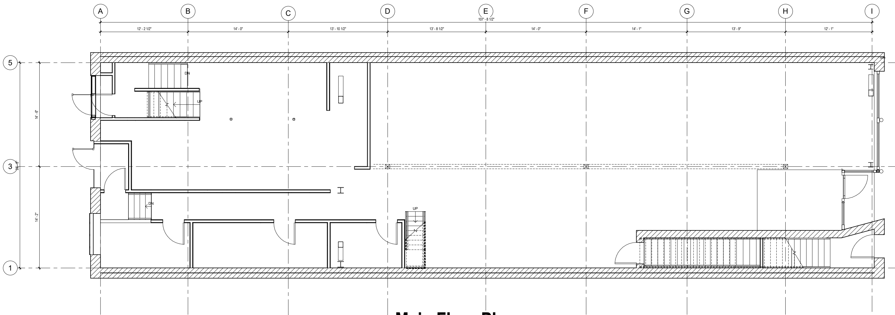
Main Floor Plan
